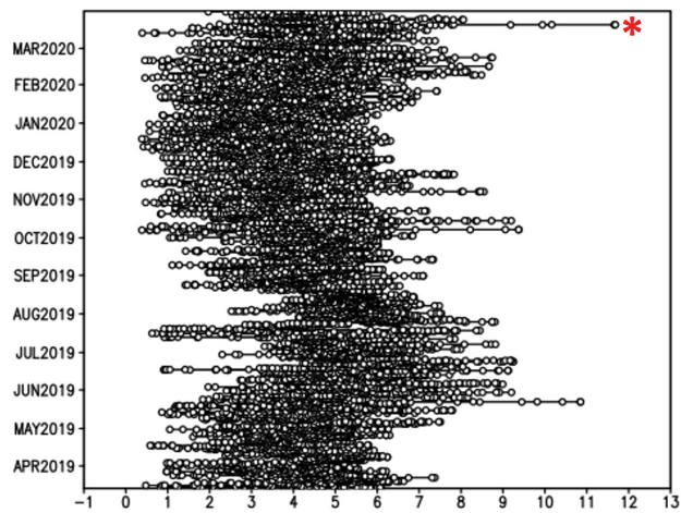
Fig 3b. The Hovmoller diagram of the longitude-averaged maximum hourly surface wind speed 0.5 \times 0.625 deg. [MERRA-2 model M2T1NXFLX v5.12.4] \text{m s}^{-1} over 2019-03-14 00Z - 2020-03-30 23Z, Region 8.5982E, 4.2737N, 8.9525E, 4.7269N (asterix= outlier value)
