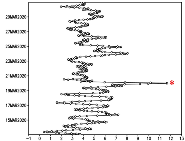
Fig 3c. The Hovmoller diagram of the longitude-averaged maximum hourly surface wind speed 0.5 \times 0.625 deg. [MERRA-2 model M2T1NXFLX v5.12.4] \text{m s}^{-1} over 2020-03-13 00Z - 2020-03-30 23Z, Region 8.5982E, 4.2737N, 8.9525E, 4.7269N (asterix= outlier value)
