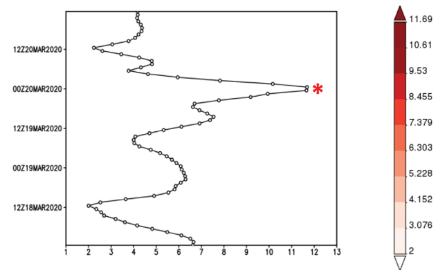
Fig 3d. The Hovmoller diagram of the longitude-averaged maximum hourly surface wind speed 0.5 \times 0.625 deg. [MERRA-2 model M2T1NXFLX v5.12.4] \text{m s}^{-1} over 2020-03-18 00Z - 2020-03-20 23Z, Region 8.5982E, 4.2737N, 8.9525E, 4.7269N (asterix= outlier value)
