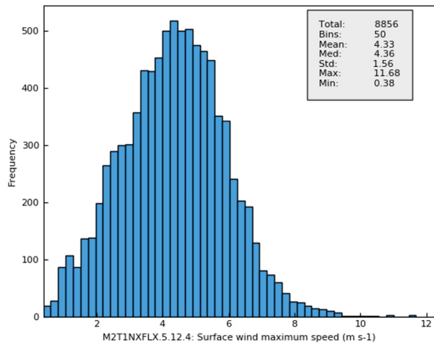
Fig 3a. Histogram of the maximum hourly surface wind speed 0.5 \times 0.625 deg. [MERRA-2 Model M2T1NXFLX v5.12.4] \text{m s}^{-1} over 2019-03-18 00Z - 2020-03-20 23Z, Region 8.5982E, 4.2737N, 8.9525E, 4.7269N
